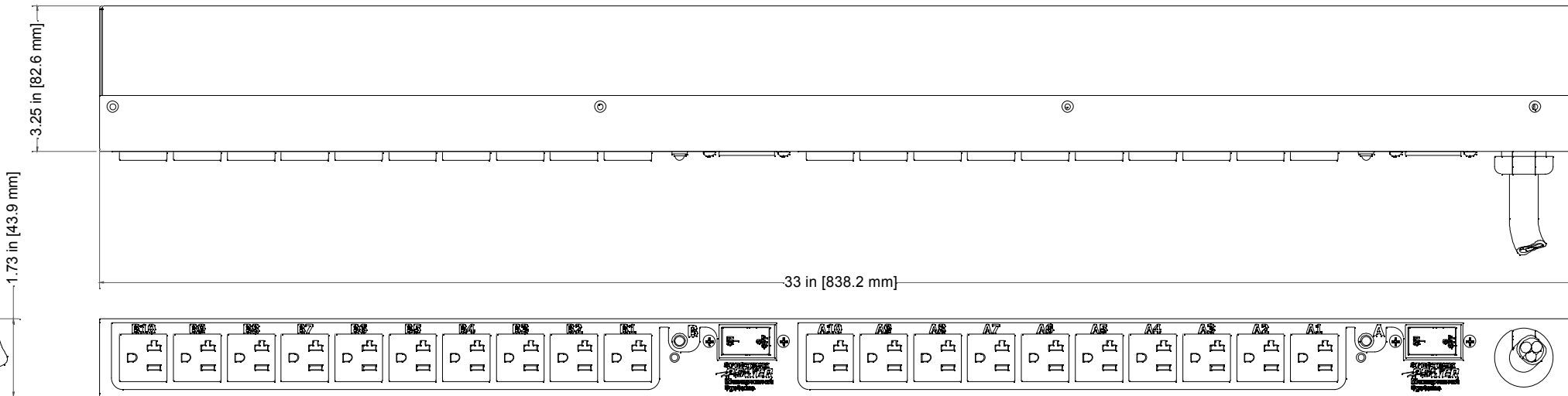
L5-30P PLUG END
